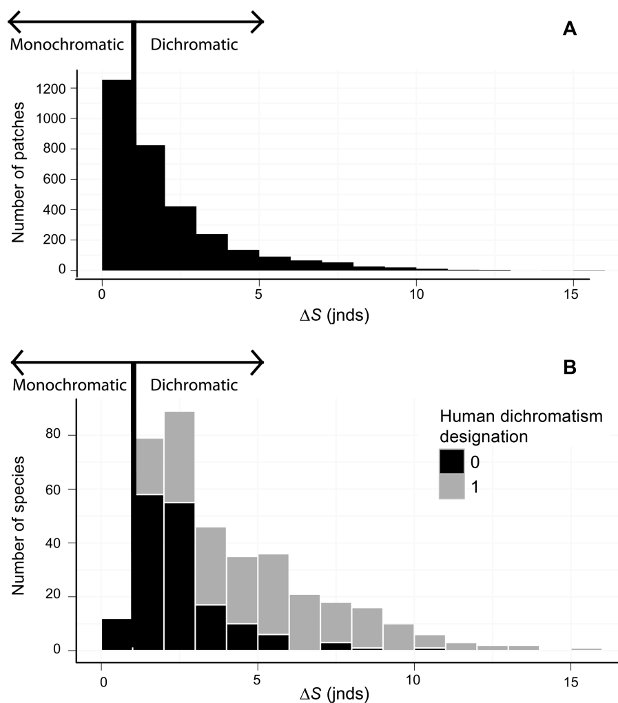
FIG. 2. (A) Distribution of \Delta S values across all patches measured. (B) Distribution of the highest \Delta S measured for each species. \Delta S is measured in just noticeable differences (jnds), and a value greater than one indicates a perceivable difference.
